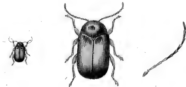
Cryptocephalus nitens.
